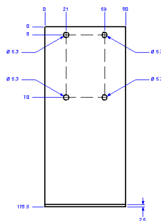
Mounting angle
